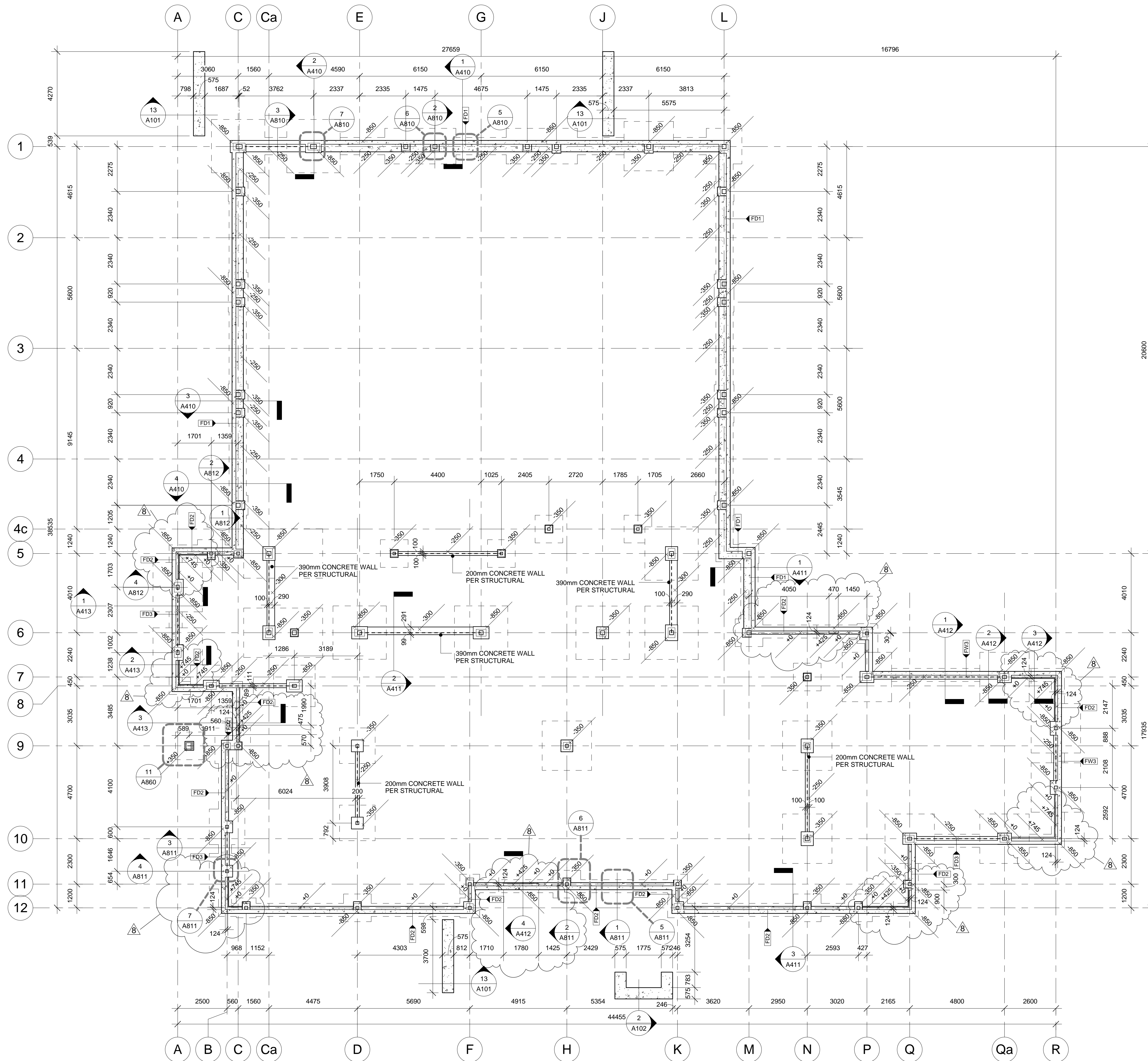
1 FOUNDATION PLAN A200 1:100
